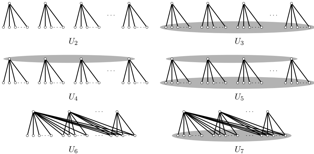
Figure 1: The universal graphs.
