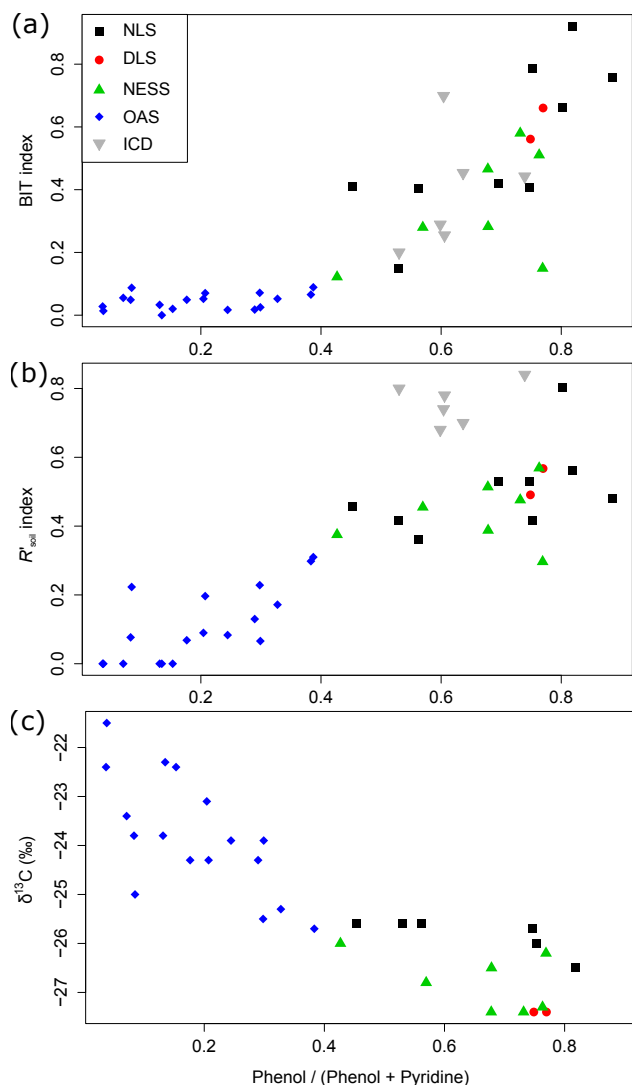
Figure 5. The phenol/pyridine ratio plotted against (a) BIT, (b) R'_{\text{soil}} and (c) \delta^{13}\text{C}_{\text{COC}} . In each case there is a strong correlation between the proxies. (DLS: Dmitry Laptev Strait; NLS: nearshore Laptev Sea; NESS: nearshore East Siberian Sea; OAS: offshore Arctic shelf).
