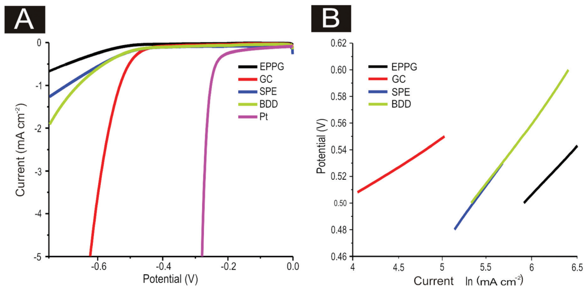
Fig. 4 (A) LSV of 1267 \text{ ng cm}^{-2} 2D \text{MoS}_2 nanosheet modified EPPG, GC, SPE, BDD electrodes and an unmodified Pt electrode showing the onset of the HER. In all cases, scan rate: 25 \text{ mV s}^{-1} (vs. SCE). Solution composition: 0.5 \text{ M H}_2\text{SO}_4 . (B) Tafel analysis; potential vs. natural log (ln) of current density for Faradaic section of the LSV presented in (A).
