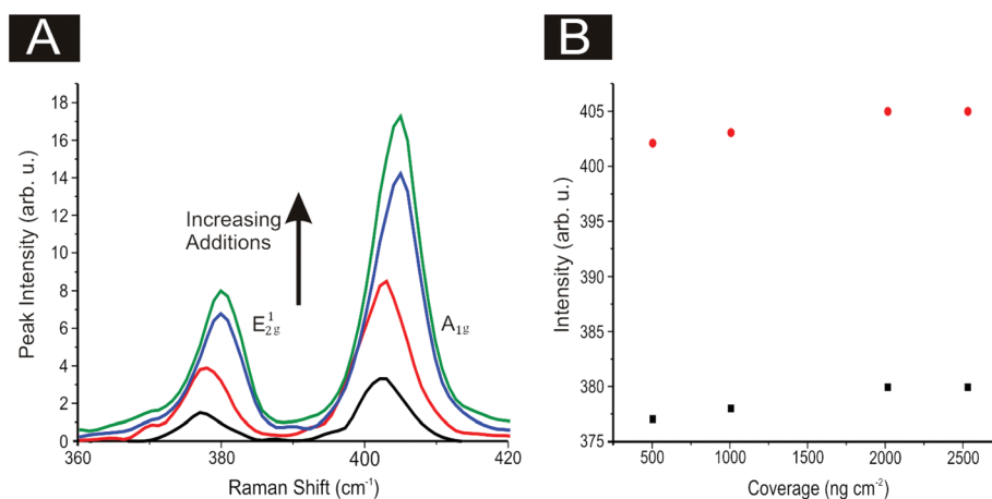
Fig. 5 (A) Raman spectra peak intensity and position for 504 (black), 1009 (red), 2019 (blue) and 2533 (green) \text{ng cm}^{-2} 2D \text{MoS}_2 nanosheet modifications on SPEs. (B) Depicts 2D \text{MoS}_2 nanosheet coverage plotted against Raman peak intensity for \text{E}_{2g}^1 (black) and \text{A}_{1g} (red) vibrational bands, showing a constant peak distance of 24.7 \text{ cm}^{-1} at all coverages.
