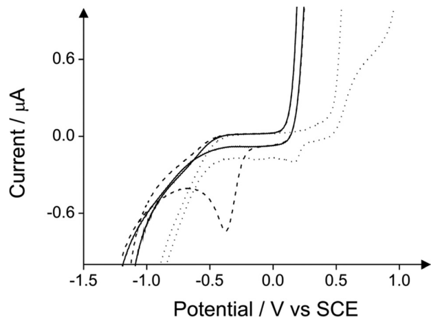
Fig. 12 Cyclic voltammetric responses of the BDDE from using 400 mg L -1 4-aminoantipyridine (solid line), 400 mg L -1 4-aminoantipyridine and 10 mg L -1 2-chlorophenol (dashed line) and 10 mg L -1 2-chlorophenol into a drinking water (tap) sample adjusted to pH 10. Starting potential: -1.2 V, first vertex potential: +1.0 V, end potential: -1.2 V. Scan rate: 50 mV s -1 .
