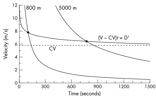
Figure 1 Schematic example of individual velocity-time ( V-t ) curve. Distance curves to 800 m and 5000 m are also shown. The point of intersection of these curves corresponds to the runner's maximal average velocities (y axis) and/or best possible performance times (x axis) for the distances. CV, Critical velocity; D' , distance curvature. Running velocities above the individual V-t curve are unsustainable because of metabolic limitation, and running at a velocity below the CV for any part of a race will result in a suboptimal performance. See text for further details.
