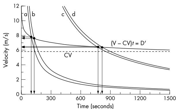
Figure 2 Schematic example of the effect of running further than the actual race distance on the time to complete the race. Curves a and c are the distance curves to 800 m and 5000 m respectively; curves b and d are the distance curves that may pertain if the athlete did not run the shortest possible distance (by running wide on the bends in track races, for example). Note that the points of intersection of the distance curves and the V-t curve shift downwards and to the right, resulting in the athlete maintaining a lower average velocity ( y axis) and thus taking more time ( x axis) to complete the race. Note also that, because of the shape of the individual V-t curve, a small reduction in average velocity results in a relatively large increase in race time as race distance increases.
