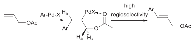
Scheme 2. Source of the high observed regioselectivity.
