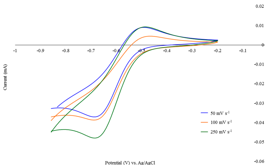
Figure 1. Cyclic voltammograms of compound 4 in \text{CH}_3\text{CN} (0.1 M tetrabutylammonium perchlorate (TBAP)) recorded at scan rates of 50, 100 and 250 \text{mV s}^{-1} at a glassy carbon electrode at 20 ^\circ\text{C} .
