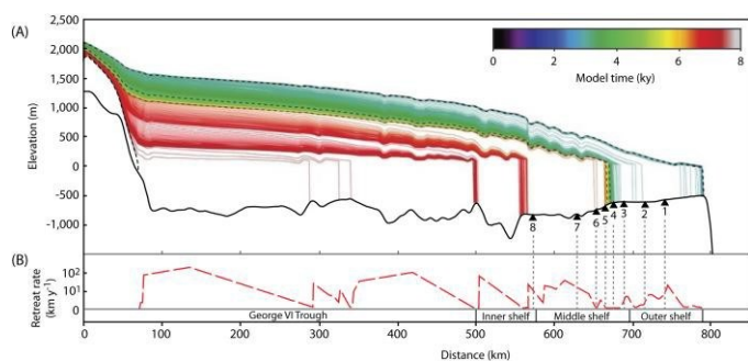
Fig. 15. Modelled ice stream retreat characteristics along the Marguerite Bay ice stream (western Antarctic Peninsula), illustrating the comparative stability of the grounding-line on topographic highs and on reverse bed slopes (where the trough narrowings). (A) Along-flow profiles of surface elevation and terminus positions. Coloured lines reflect ice surface profiles at 5-year intervals, over an 8000-year period. Dotted black lines show the ice surface every 2000 years. The along-flow bed geometry is shown by the solid black line. (B) Modelled grounding-line retreat rate
