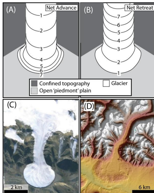
Fig. 14. Illustration of the impact variations in valley width can have on glacier margin stability and moraine location. (A) Schematic planview of different phases of glacier growth during net advance (ELA lowering). Numbers reflect stages of growth and illustrate how glaciers confined to narrow basins advance rapidly (stages 1-3), but upon emerging from valley confines, expand laterally, leading to comparative stability (stages 3-7). (B) Schematic planview of different phases of glacier retreat. Numbers reflect stages of retreat and illustrate how piedmont glacier retreat is
