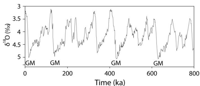
Fig. 8. Benthic \delta^{18}\text{O} record (considered a proxy for global ice volumes) covering the past 800,000 years (from Lisiecki and Raymo, 2005). These data are used by Anderson et al. (2012) to support the argument that, even when climatic conditions (as reflected by global ice volumes) remain essentially the same from one glacial maximum (GM) to the next, ice masses can experience a reduction in areal extent over successive glacial cycles because glacial erosion skews basin topography toward lower altitudes over time (i.e., erosional feedback).
