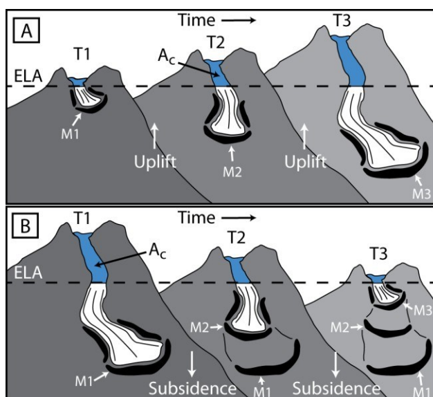
Fig. 5. Illustration of the impact mountain uplift and subsidence (or denudation) can have on glacier extent, and therefore moraine location, under uniform climatic conditions (fixed ELA). (A) Where uplift occurs between phases of glaciation (marked by time-steps T1, T2, and T3), glacier length progressively increases. At each time-step, maximum ice extent is marked by a deposited moraine (M1-3). In this scenario, only the outermost moraine (i.e., M3) is preserved, as older moraines are destroyed by obliterative overlap. (B) Where upland subsidence (or denudation) occurs between phases of glaciation, glacier length progressively decreases, and a detailed record of different-aged
