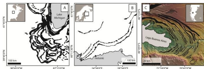
Fig. 2. Examples of extensive, arcuate end moraines. (A) Moraines marking the southern extent of the Lake Michigan lobe of the Laurentide Ice Sheet, between 22 and 13.5 ka (redrawn from Frye and Willman, 1973). (B) The Salpausselkä (I, II, III), North Karelia, Koitere, and Pielisjärvi end moraines, demarcating former ice sheet extent in
