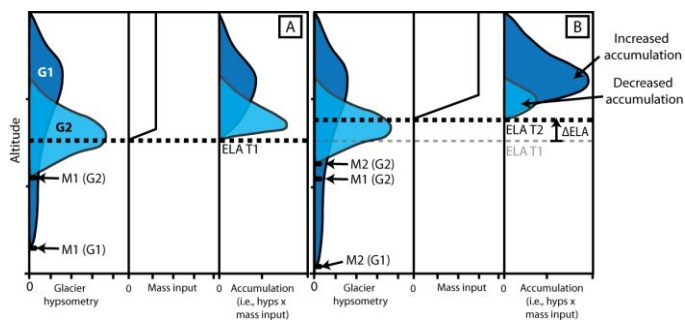
Fig. 4. Schematic illustration of how glacier hypsometry (as controlled by accumulation area topography) can regulate the nature of glacier response to fluctuations in climate. In this example, a shift from (A) cryo-arid conditions with comparatively low ELA but low mass turnover (i.e., nondynamic glaciers) to (B) warmer, wetter conditions with slightly higher ELA (rise of \sim 120 m) and greater mass turnover (more dynamic glaciers), can lead a glacier (G1) with a high altitude source area to advance, whilst a lower-altitude glacier (G2) recedes. G2 reaches its maximum extent during phase A, whilst G1 reaches its maximum extent during phase B. Thus, accumulation area topography results in asynchronous glacial maxima and very different moraine records preserved in each basin. For example, the moraine record preserved by G1 will reflect ice extent during the more recent, higher ELA, phase of advance, whilst G2 may preserve a more detailed moraine record, reflecting ice extent before and after the increase in ELA. Figure adapted from Pratt-Sitaula et al. (2011).
