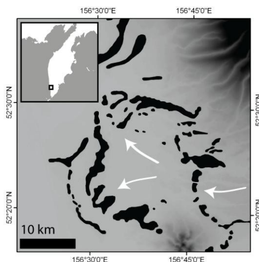
Fig. 17. Moraine sequences in southwestern Kamchatka. Individual moraine segments have indistinct plan morphology but appear arcuate when viewed as a continuous sequence. White arrows show inferred palaeo ice-flow directions. Mapping from Barr and Clark (2012a,b).
